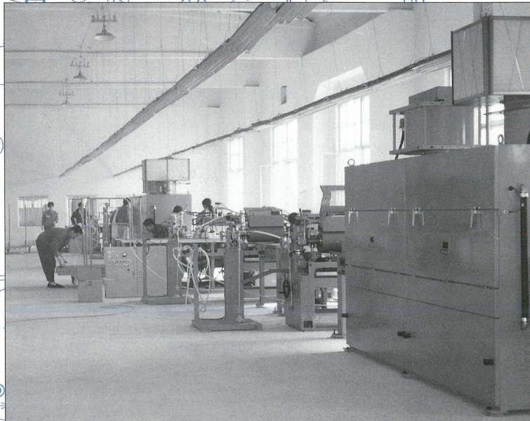
UV coating/drying line (base & top coating) No solvent required, i.e. no setting time. Thus the line needs minimum space.
