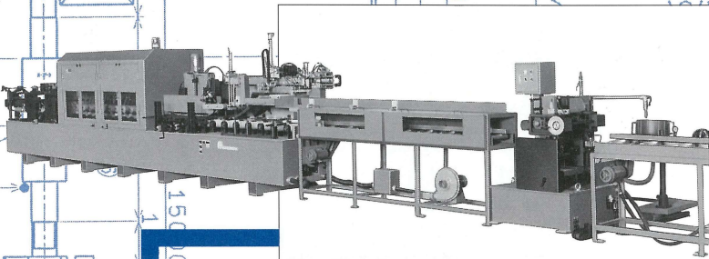
Radio-frequency veneer roll press laminator Laminating veneers on base material to make fine laminated wood in one-pass operation.
