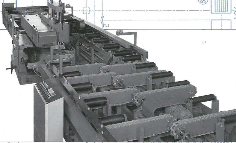
Veneer slicer, SL-350V with conveyor system Superior veneer quality realized by "lengthways slicing system"
