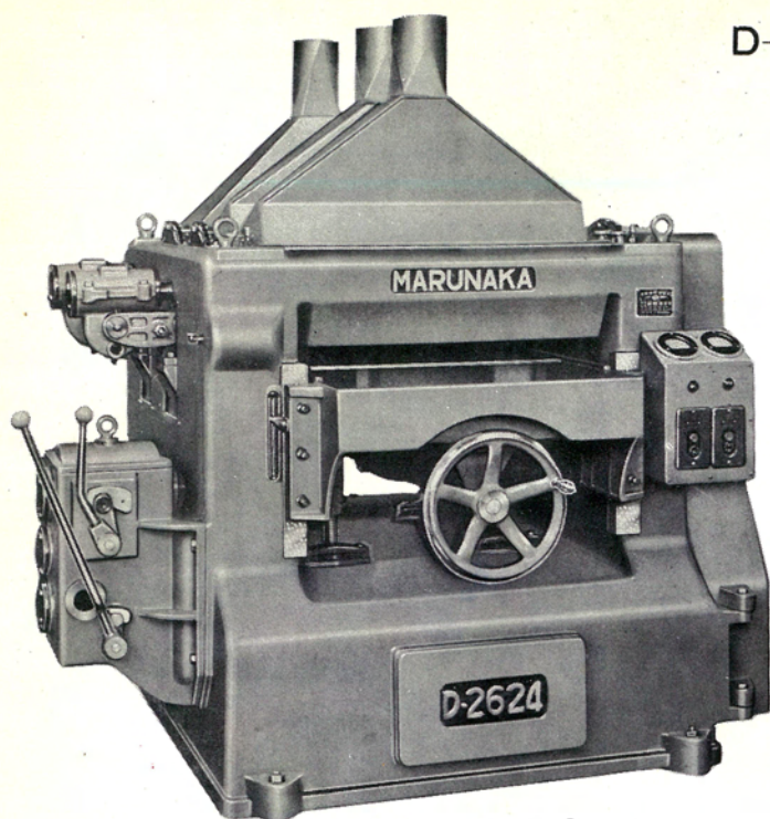
D-2624 Drum Sander
