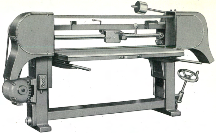
BP-05 1500mm Belt Sanding Machine
